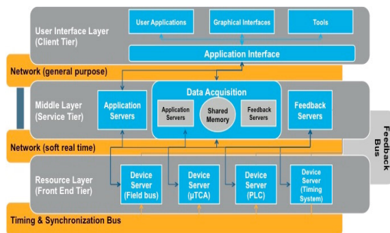
Figure 2: Accelerator control system layout with three layers and integrated data acquisition system on the middle layer.
