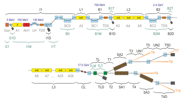
Figure 1: Schematic overview of the overall European XFEL accelerator with injector (I1), linear accelerator tunnel (L1 – L3), the collimation and distribution section (CL and TL) and the various SASE beam lines with its undulators (T1 – T10, SA1 – SA3).
